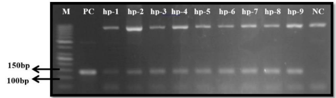
Fig. 3. Electrophoretic of PCR products of 130 nucleotide fragment of TuMV CP gene in transgenic canola RGS003 plants. 130 nucleotide fragment at the below and 800 nucleotide fragment of Acc gene of canola as PCR control at the above. (M: GenRuler™ 50bp DNA ladder, Fermentas; pFGC-CP-S as a pFGC-CP-S, pFGC-CP-AS and pFGC-CP-hp as a sense, antisense and hairpin.
