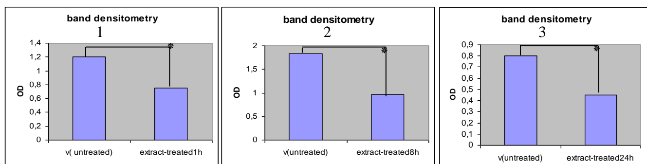
Fig. 2: Semi-quantitative analysis of the virus genome contents before and after treatment with the extract at 3 time points: 1) 1h, 2) 8h, 3) 24h.
