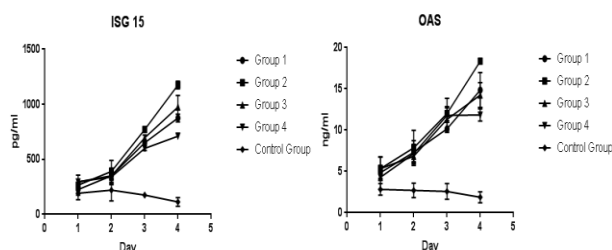
Fig. 3. The levels of OAS and ISG15 proteins in PBMCs after treatment with IFN- \alpha 2a. The PBMCs were isolated from treatment-naïve HCV-infected patients and cultured in 96-wells plate in the presence of different concentrations of IFN- \alpha 2a for 96 h. The levels of OAS and ISG15 were measured in the culture supernatants by ELISA.
