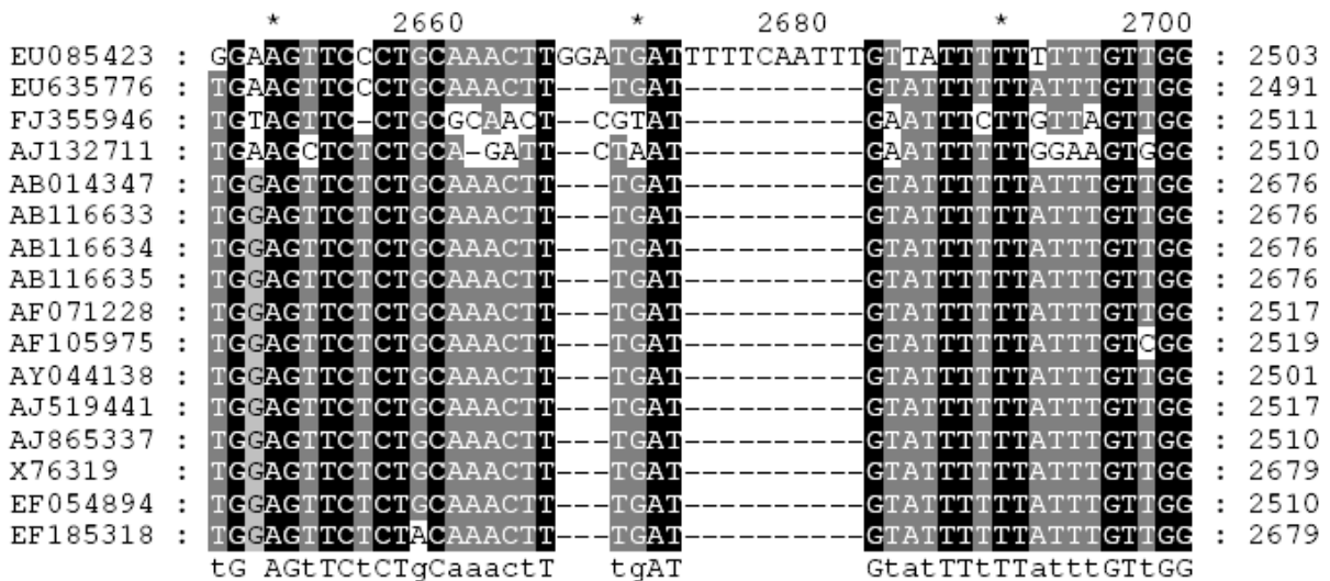
Fig. 4. The nucleotide alignment of TYLCV showing two insertion parts in TYLCV-Ir2 that located in C1 ORF.
