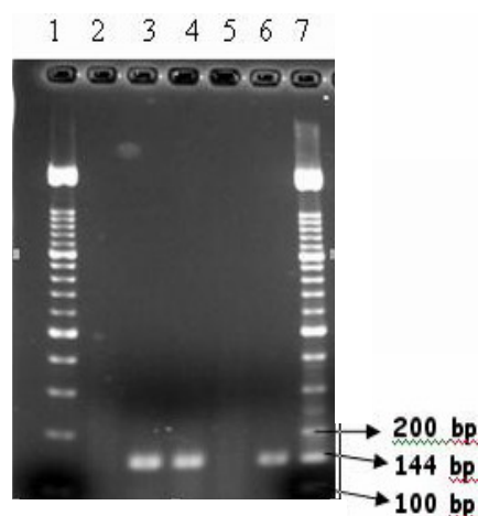
Fig. 2. Agarose gel electrophoresis (2%) following RT-PCR of CSFs for enteroviruses. Tracks 1 and 7 show 100 bp DNA ladder. Line 2 indicates negative control. Line 3 belongs to positive control (sabin vaccine). Line 4 and 6 indicate 2 positive CSF samples, and line 5 demonstrates a negative CSF sample result.
