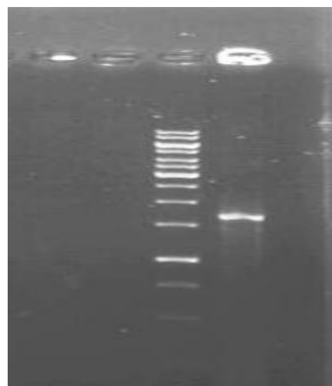
Fig. 1. Electrophoresis gel analysis of F gene (1650 bp) RT-PCR products, Lane 1: negative control (blank) Lane 2: 1 Kb DNA size marker (Fermetas). Lane 3: demonstrating a thick bond of 1650bp amplicon.
