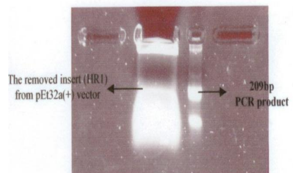
Fig. 4. Removing 209bp fragments (HR1 cDNA) from pET32a (+) vector using enzyme digestion.
