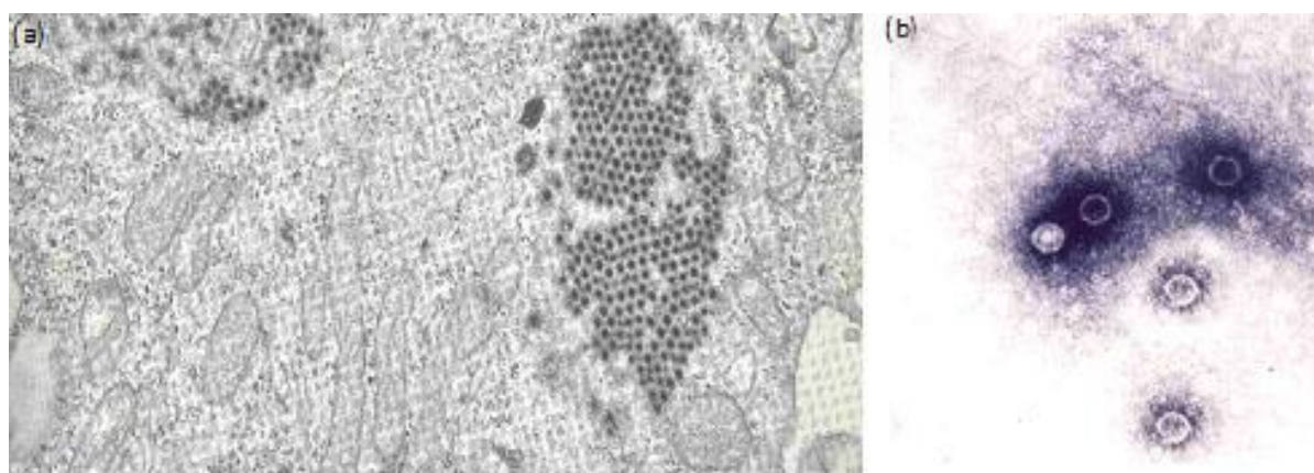
Fig. 2. (a) Electron micrograph of thin section from a reovirus infected cell superinfected with poliovirus. Many reovirus particles are present in crystal form. There is no observable poliovirus particles in the cytoplasm of infected cell ( \times 20000 ). (b) Electron microscopy of the extract of poliovirus infected control cells, prepared by the negative staining technique ( \times 120000 ).
